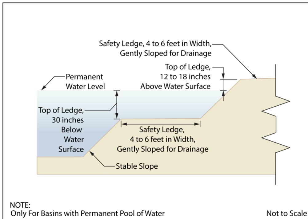
Elevation View –Basin Safety Ledge Configuration
