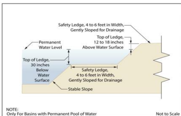
Elevation View – Basin Safety Ledge Configuration
