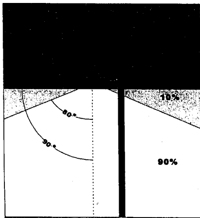
FULL CUT OFF FIXTURE Figure A
