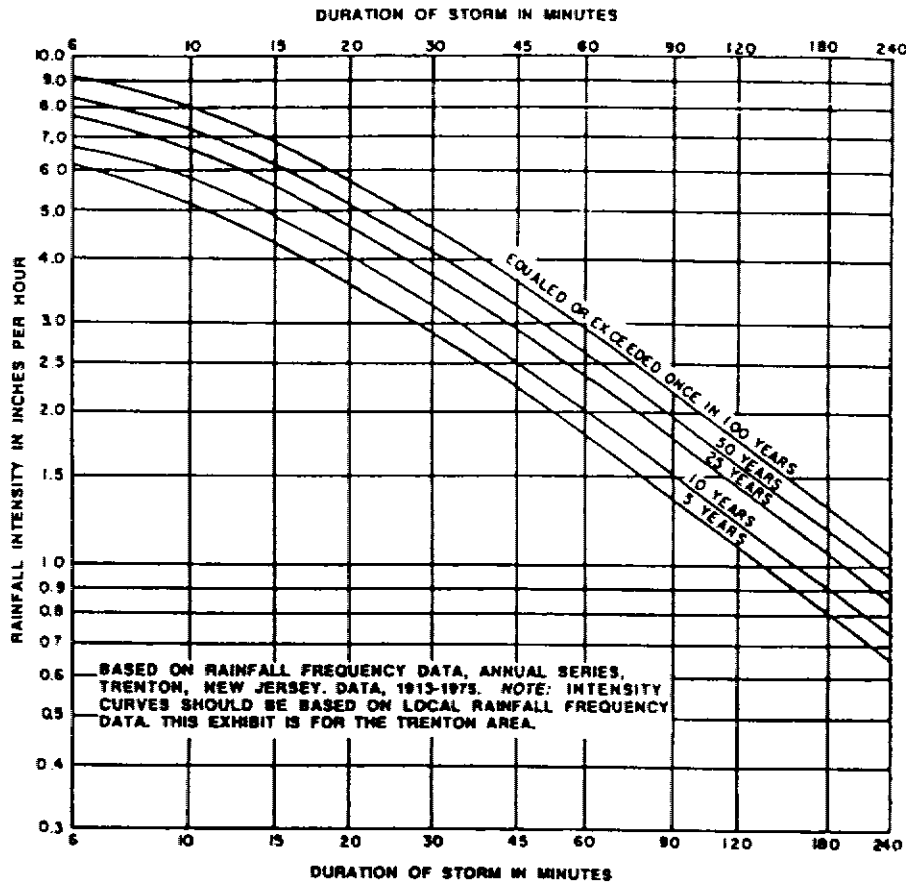
RAINFALL INTENSITY CURVES (SAMPLE)
