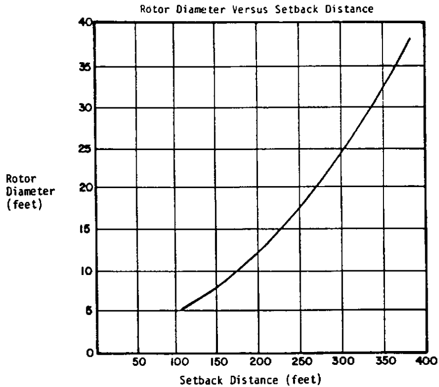
WIND TURBINE SETBACK
